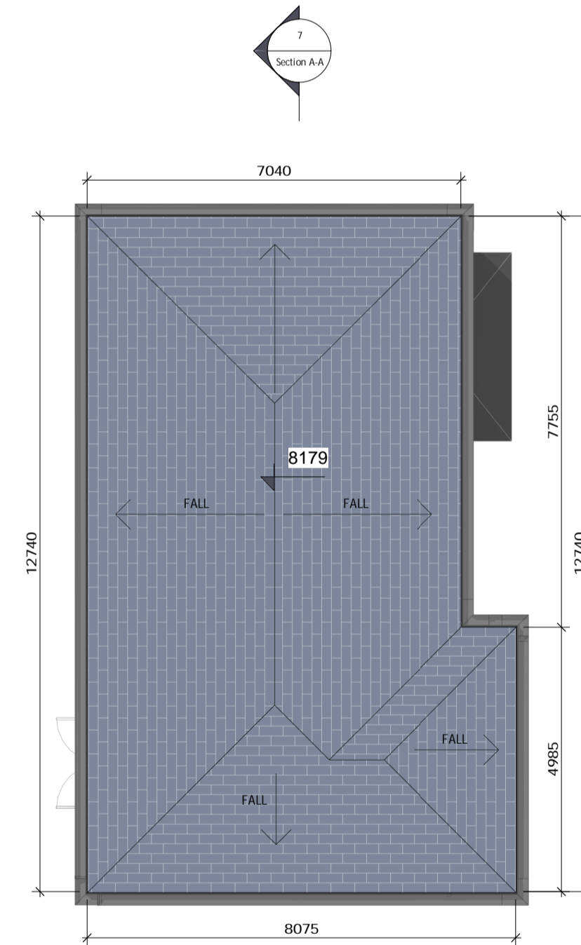
8 Roof Plan 1:100
