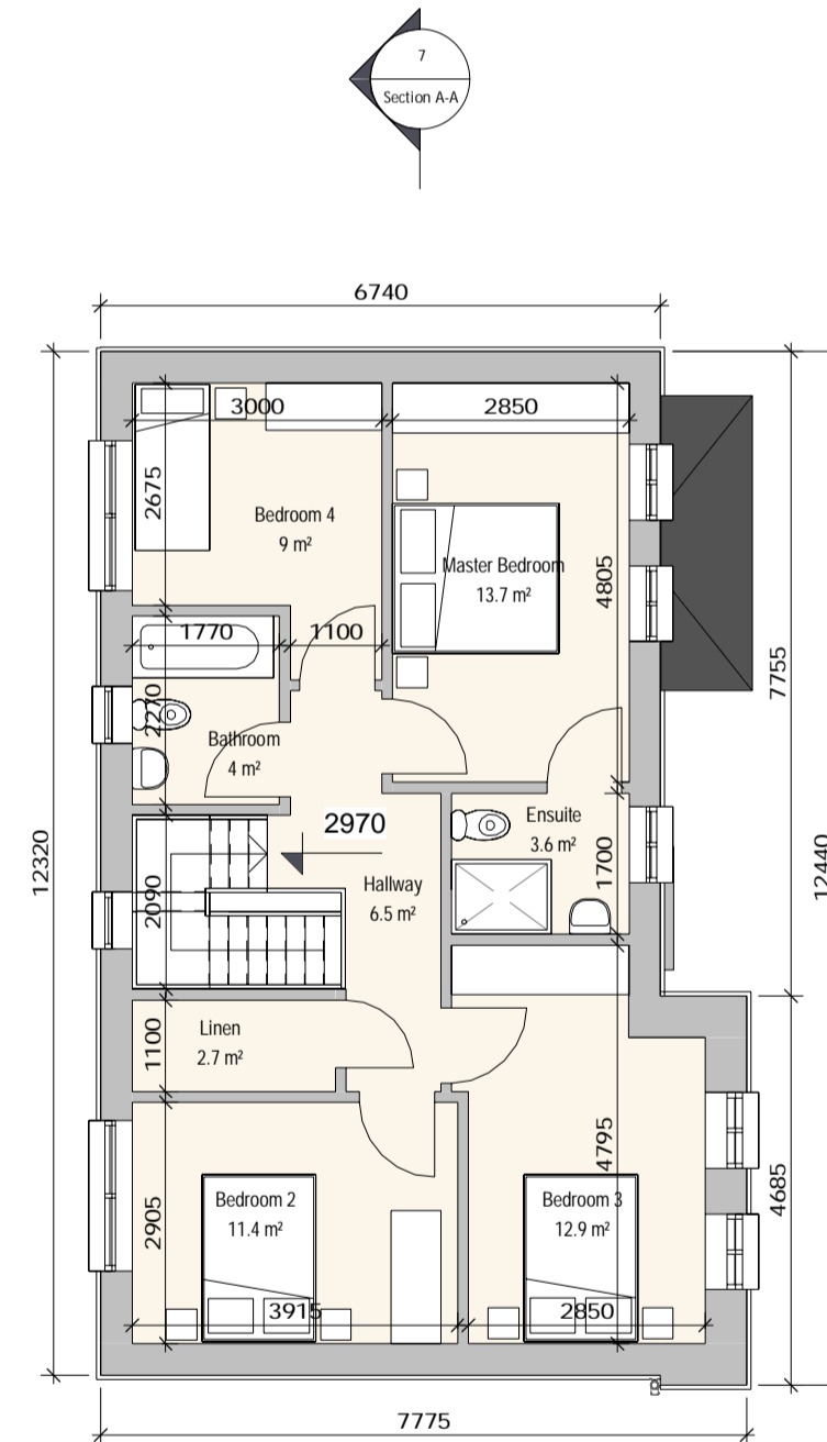
6 First Floor Plan 1:100
