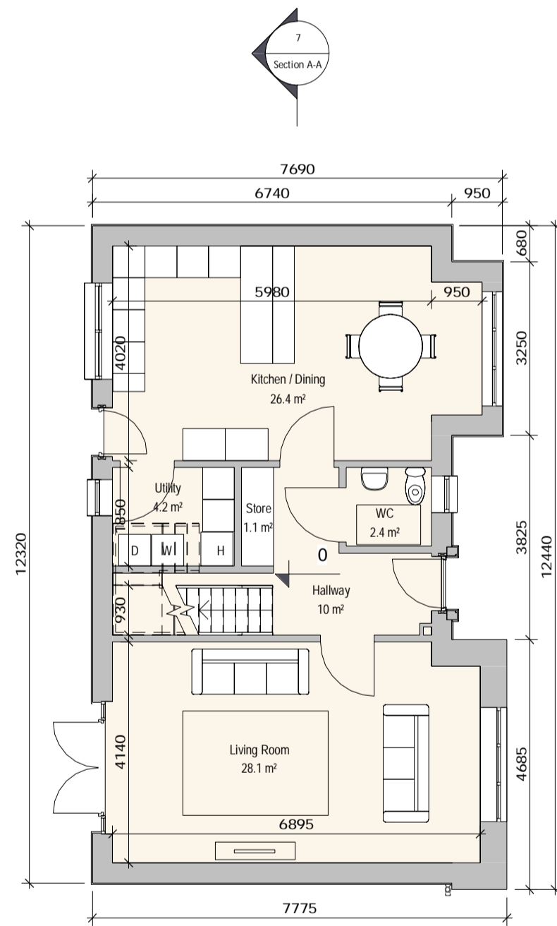
5 Ground Floor Plan 1:100
